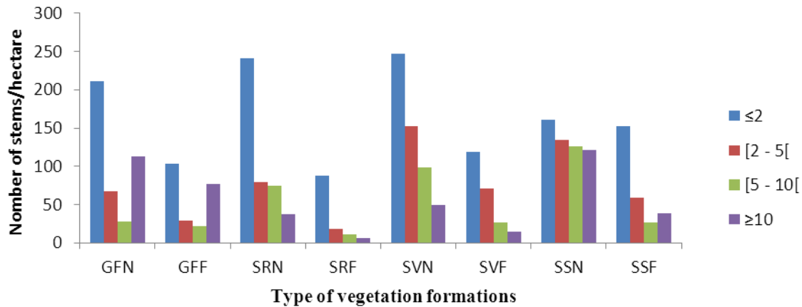
Fig. 7: Distribution of the ligneous family in height class (m). NFG = natural forest gallery, FFG= Fragmented forest gallery NRS = natural raised savannas, RSF = raised savannas fragmented, NSS= natural shrubby savannas, FSS = fragmented shrubby savannas, NWS= natural wooded savannas, FWS = Fragmented wooded savannas.
