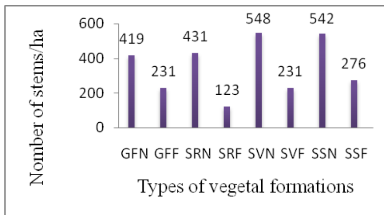
Fig. 6: Density of the various vegetal formations [NFG = natural forest gallery, FFG= Fragmented forest gallery NRS = natural raised savannas, RSF = raised savannas fragmented, NSS= natural shrubby savannas, FSS = fragmented shrubby savannas, NWS= natural wooded savannas, FWS = Fragmented wooded savannas].
