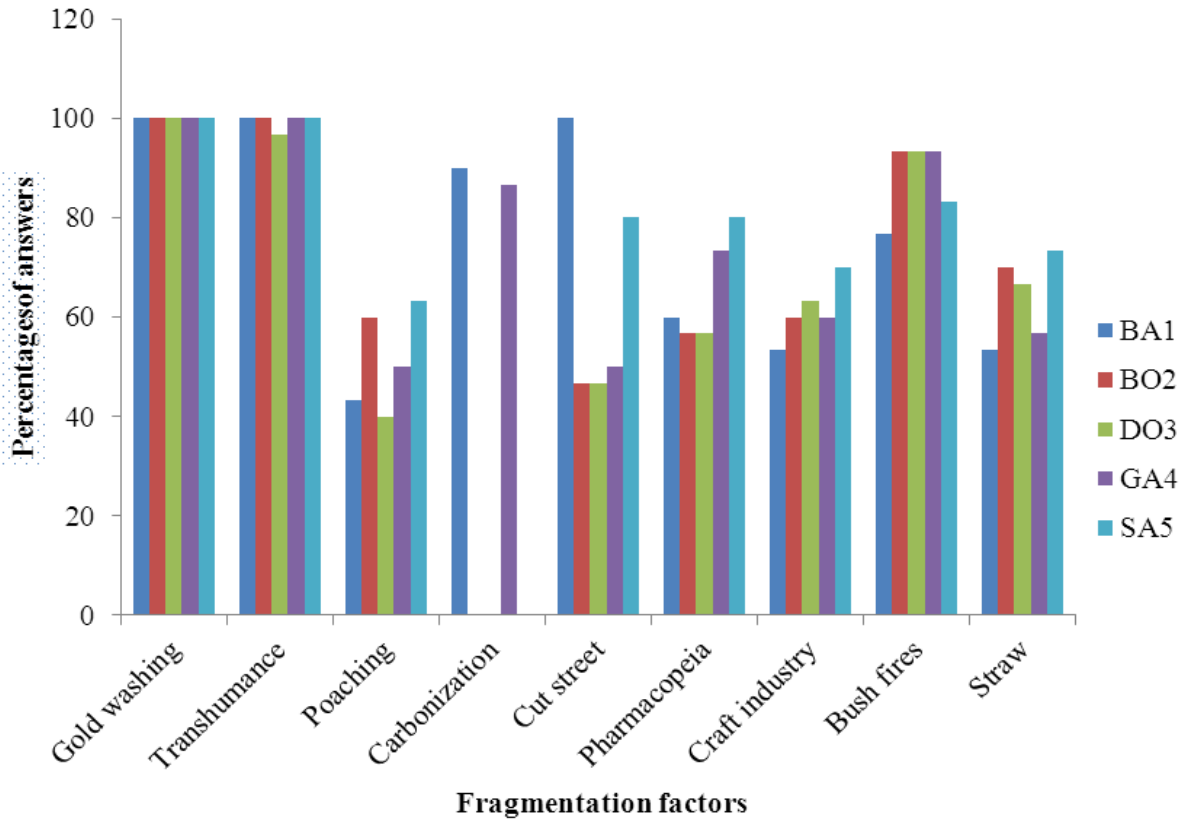
Fig. 2: Principal factors of fragmentation of the habitats of fauna in the GNP. BA1 = Bandaged; BO2 = Bouck; DO3 = Dogba; GA4 = Gamba; SA5=Sackdjé.
