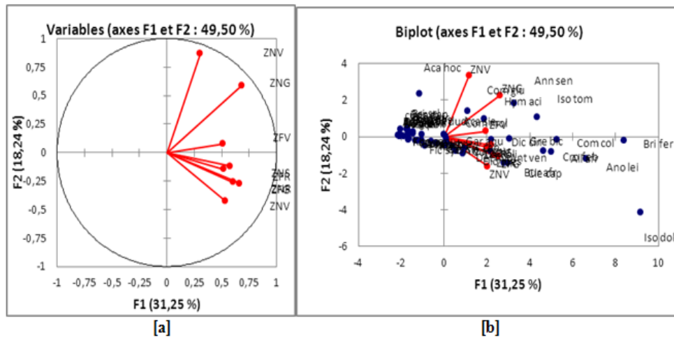
Fig. 8: ACP of the presence of species in the various statements. [a]-Distribution by types of vegetable formations; [b]- Distribution of the ligneous family in sites.
