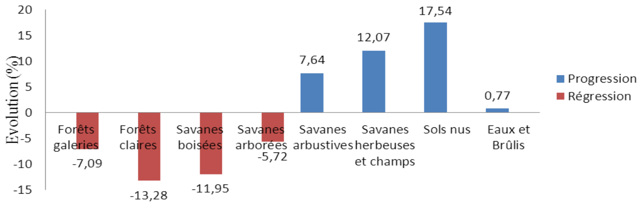
Fig. 4: Evolution rate of the fragmentation within the BNP between 2000 and 2015.
